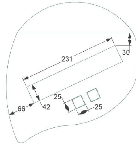
Standard softwiring provision configuration: 4 GPO or 2 GPO + USB A/C, 2 DATA prov.
